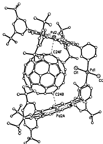
Figure 4. X-ray crystal structure of \text{Pd}_{1.5}\mathbf{2}\cdot\text{C}_{60} . The \text{Pd}2\cdots\text{C}24\text{F} distance is 2.856(10)\text{ \AA} .
