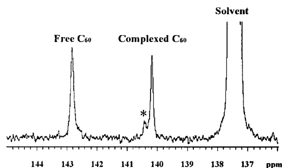
Figure 2. Low temperature ( -90\text{ }^{\circ}\text{C} ) 13 C NMR spectrum of toluene solution of 2:1 mixture of C 60 and 2 . The peak marked * is due to a small amount of Pd 2 ·C 60 .
