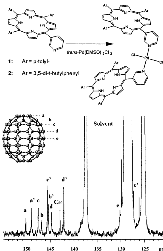
Figure 3. Low temperature ( -60\text{ }^{\circ}\text{C} ) ^{13}\text{C} NMR spectrum of toluene solution of 1.5:1 mixture of \text{C}_{70} and 2 . Resonances a'–e' are from complexed \text{C}_{70} .
